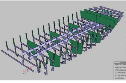
12m alloy four boat CNC construction kit
